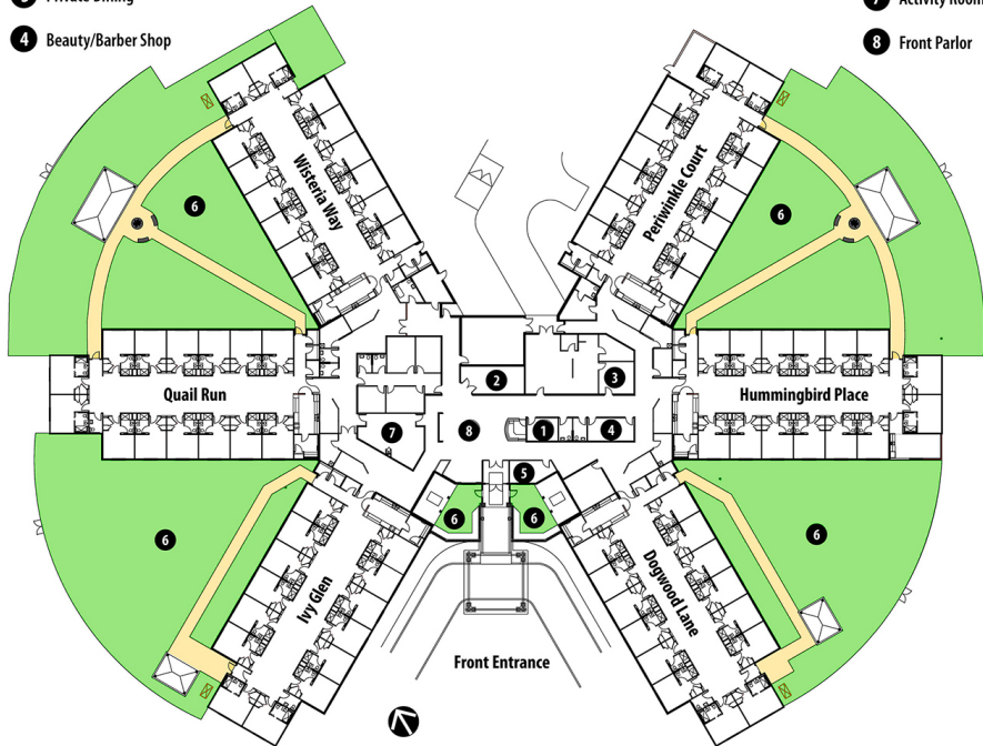
JOSEPH C. THOMAS CENTER FLOOR PLAN
